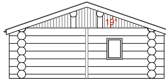
REAR ELEVATION
