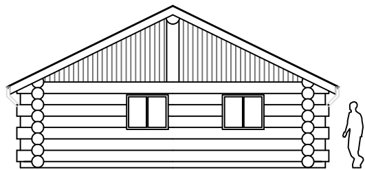
SIDE 1 ELEVATION
