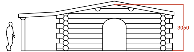
INDICATIVE SECTION
