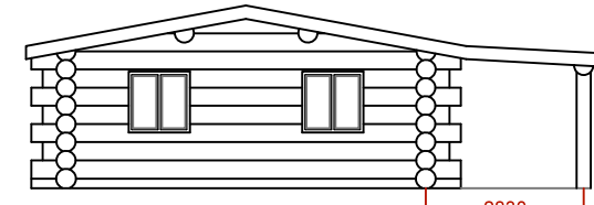
SIDE ELEVATION 2
