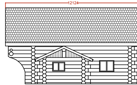
SIDE ELEVATION 1
