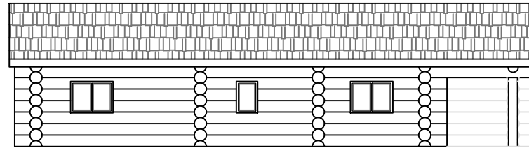
REAR ELEVATION
