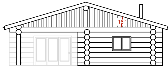
SIDE 1 ELEVATION
